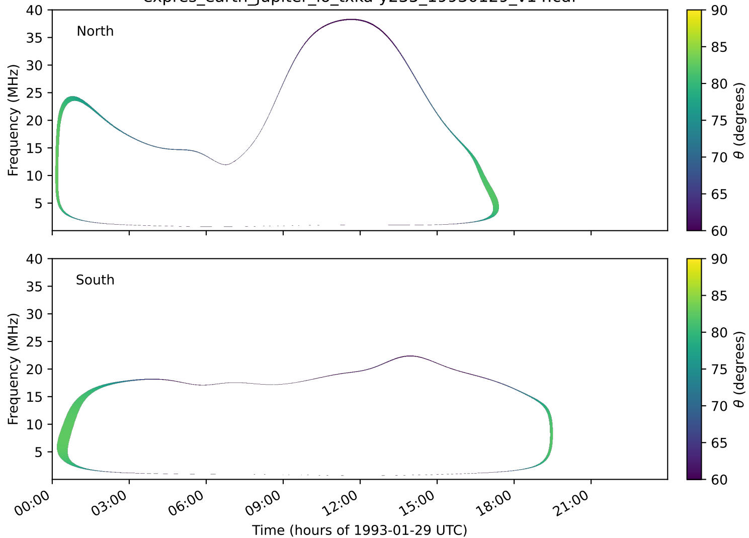
expres_earth_jupiter_io_txka-y235_19930129_v14.cdf
