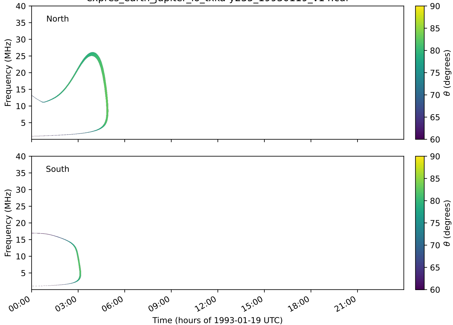
expres_earth_jupiter_io_txka-y235_19930119_v14.cdf
