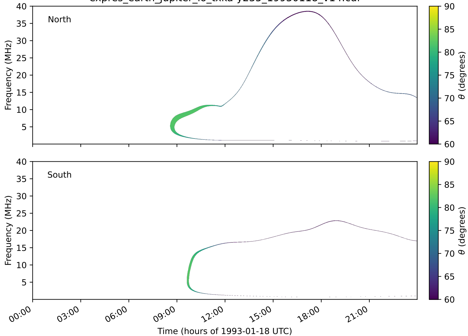
expres_earth_jupiter_io_txka-y235_19930118_v14.cdf
