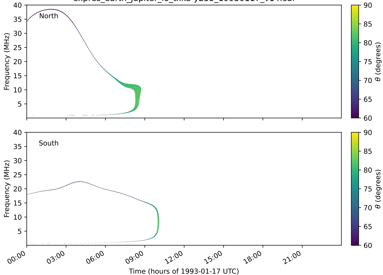
expres_earth_jupiter_io_txka-y235_19930117_v14.cdf
