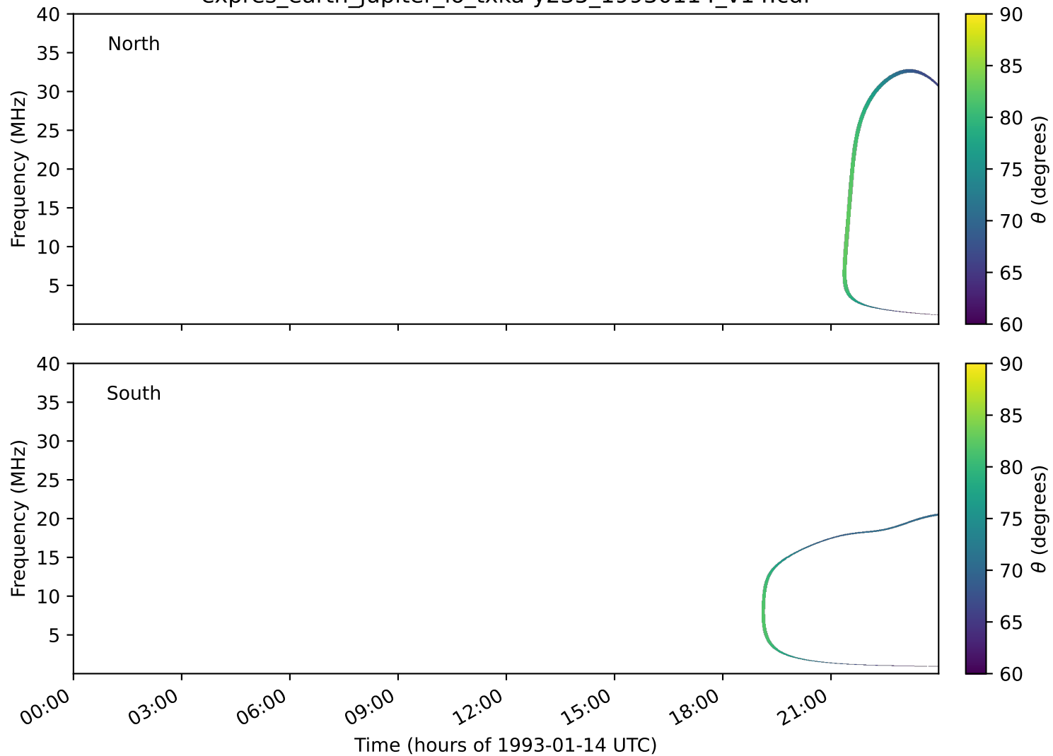
expres_earth_jupiter_io_txka-y235_19930114_v14.cdf
