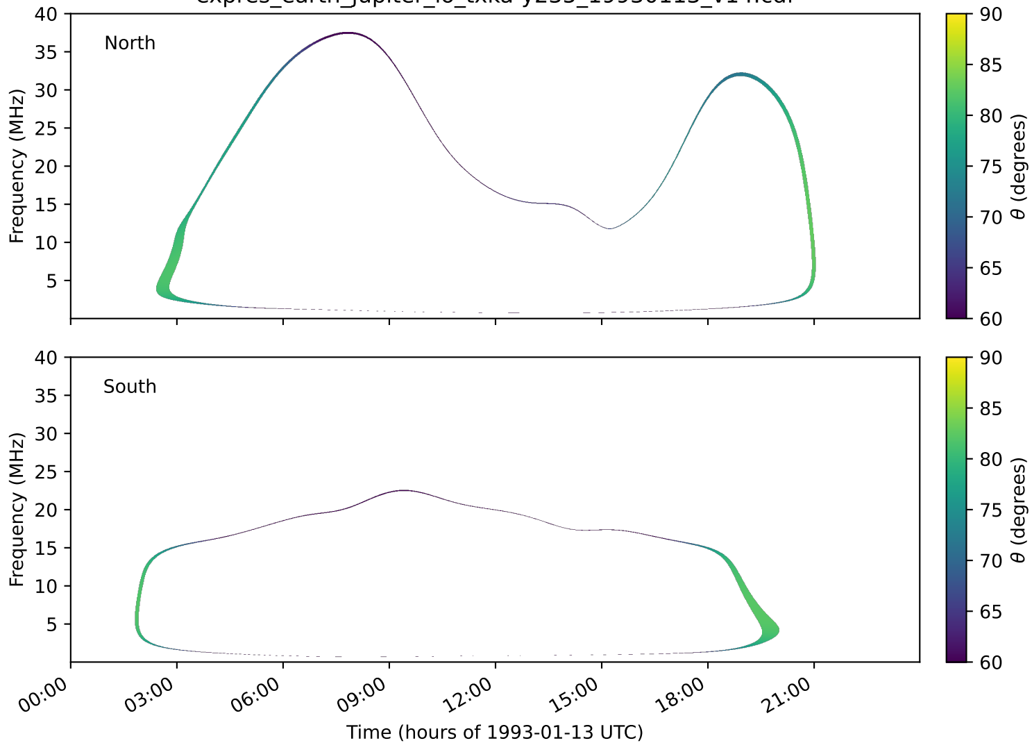
expres_earth_jupiter_io_txka-y235_19930113_v14.cdf
