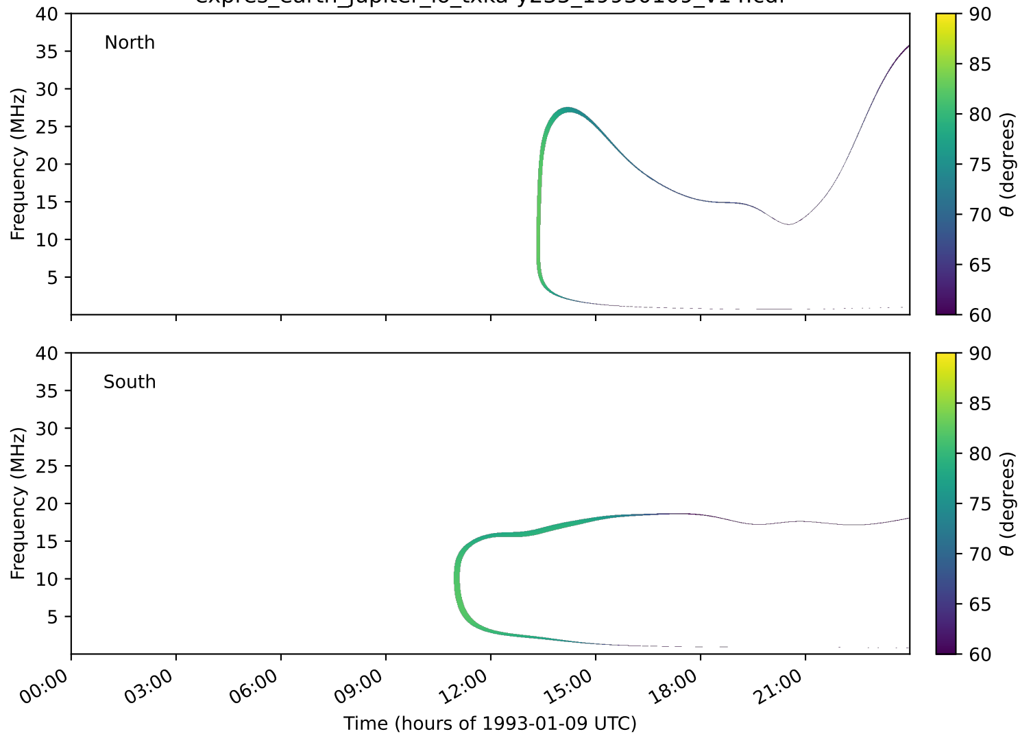
expres_earth_jupiter_io_txka-y235_19930109_v14.cdf
