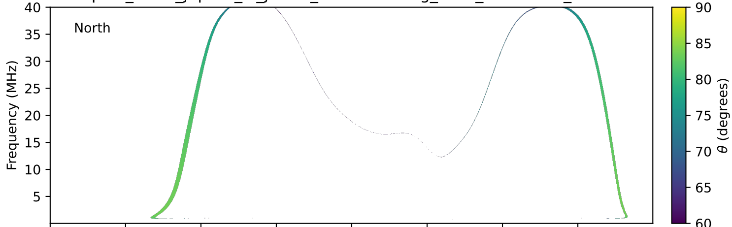
expres_earth_jupiter_io_jrm33_lossc-wid1deg_3kev_19930120_v11.cdf
