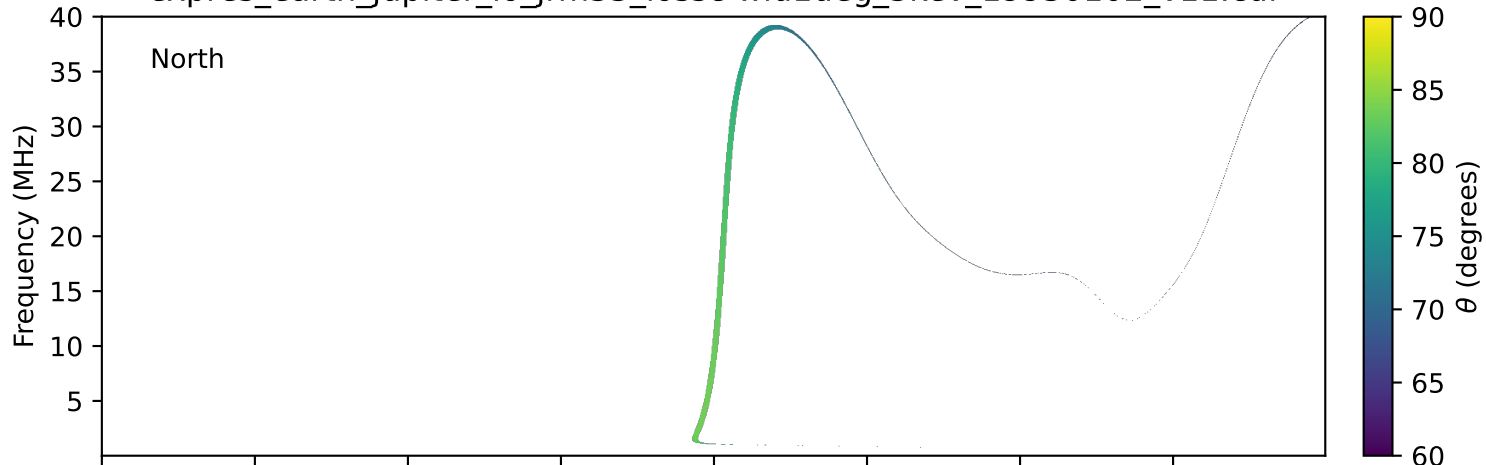
expres_earth_jupiter_io_jrm33_lossc-wid1deg_3kev_19930102_v11.cdf
