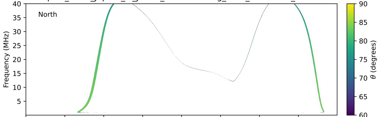
expres_earth_jupiter_io_jrm09_lossc-wid1deg_3kev_19930120_v11.cdf
