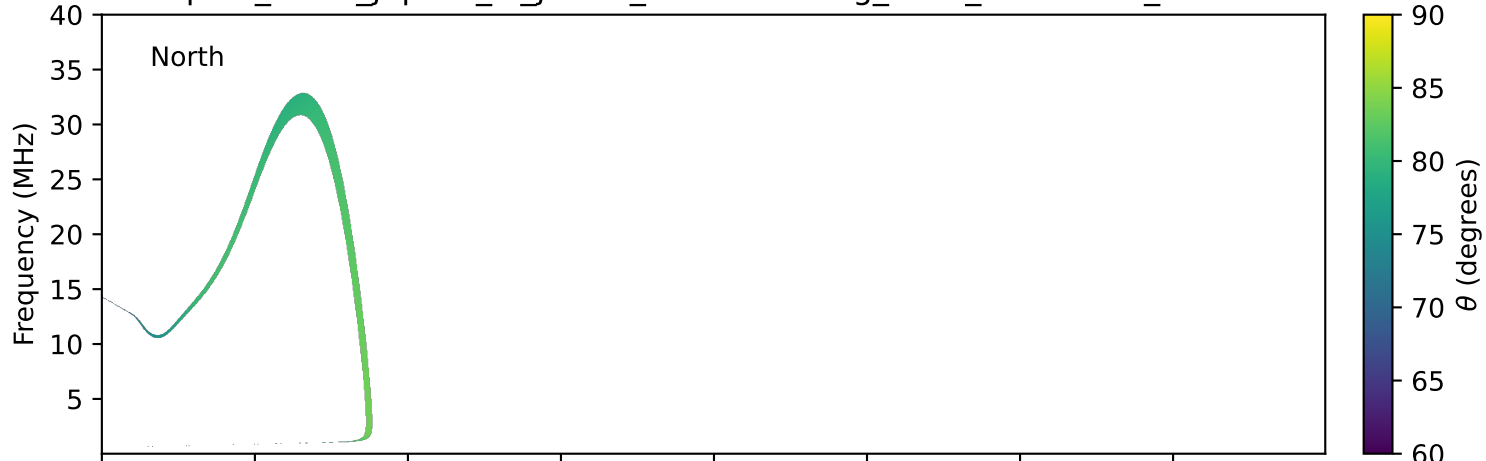
expres_earth_jupiter_io_jrm09_lossc-wid1deg_3kev_19930119_v11.cdf
