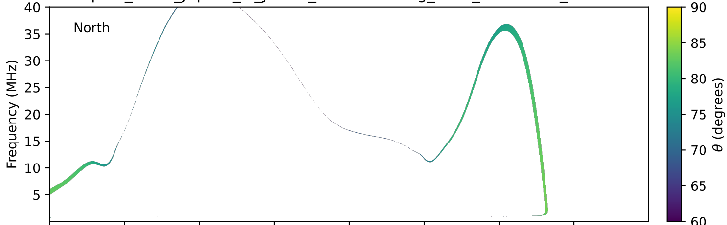
expres_earth_jupiter_io_jrm09_lossc-wid1deg_3kev_19930106_v11.cdf
