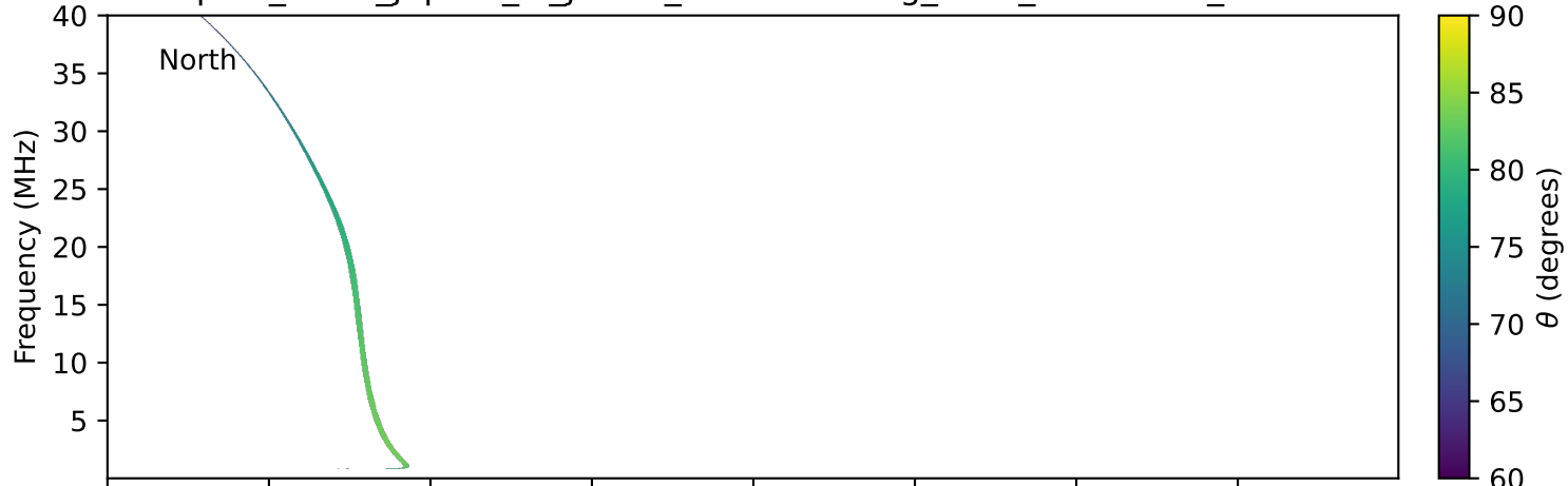
expres_earth_jupiter_io_jrm09_lossc-wid1deg_3kev_19930103_v11.cdf
