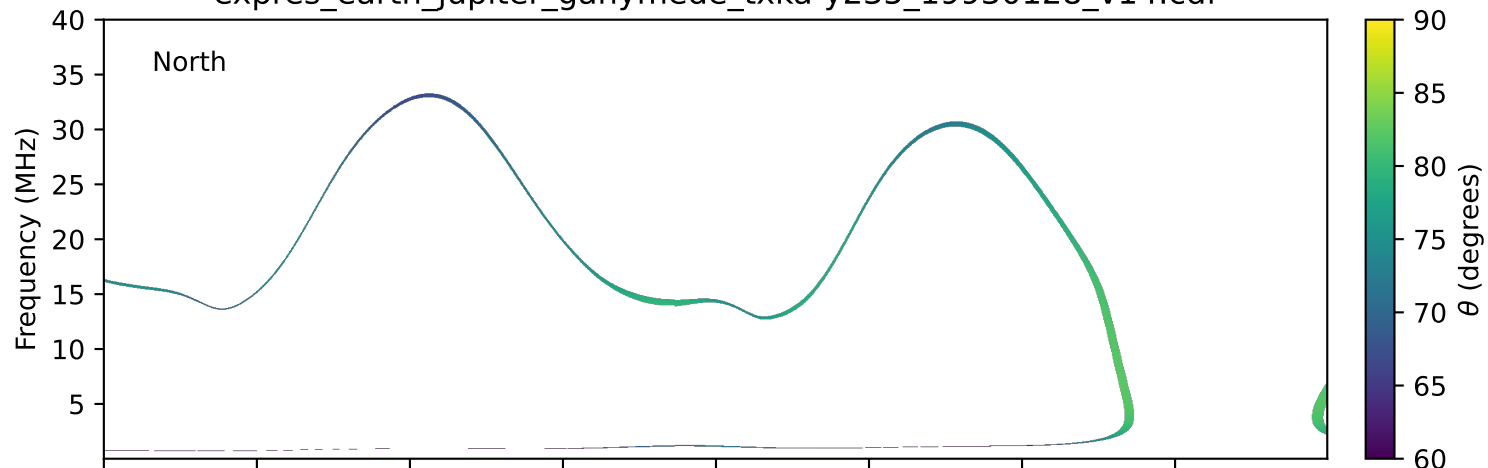
expres_earth_jupiter_ganymede_txka-y235_19930128_v14.cdf
