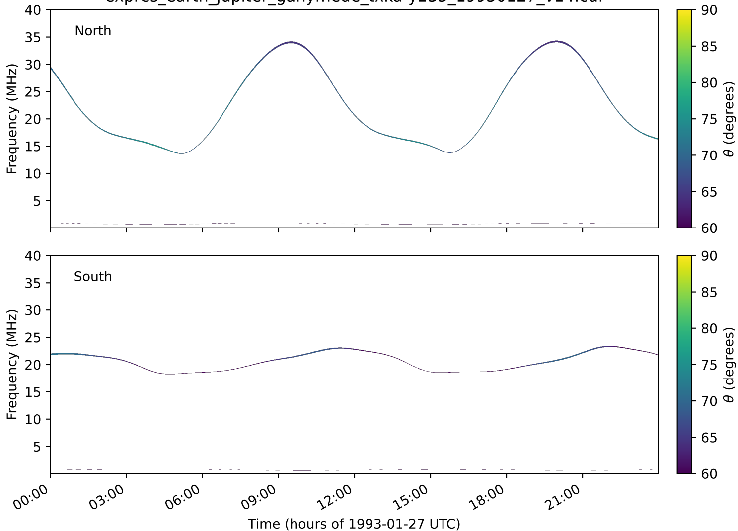
expres_earth_jupiter_ganymede_txka-y235_19930127_v14.cdf
