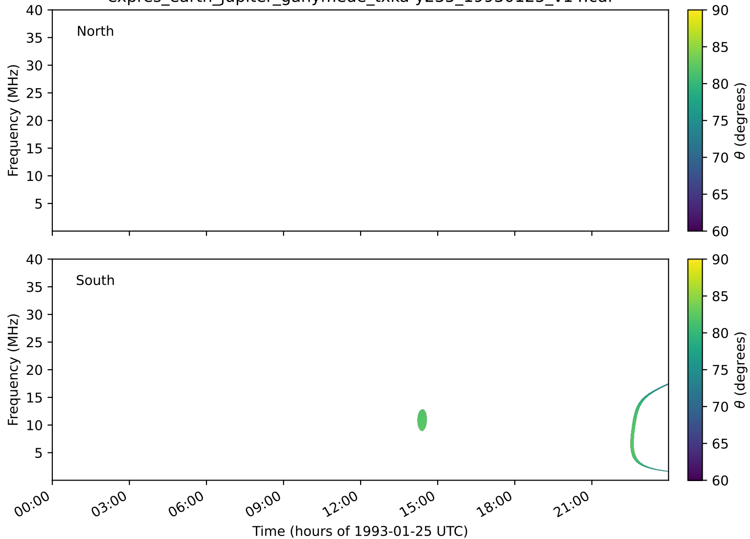
expres_earth_jupiter_ganymede_txka-y235_19930125_v14.cdf
