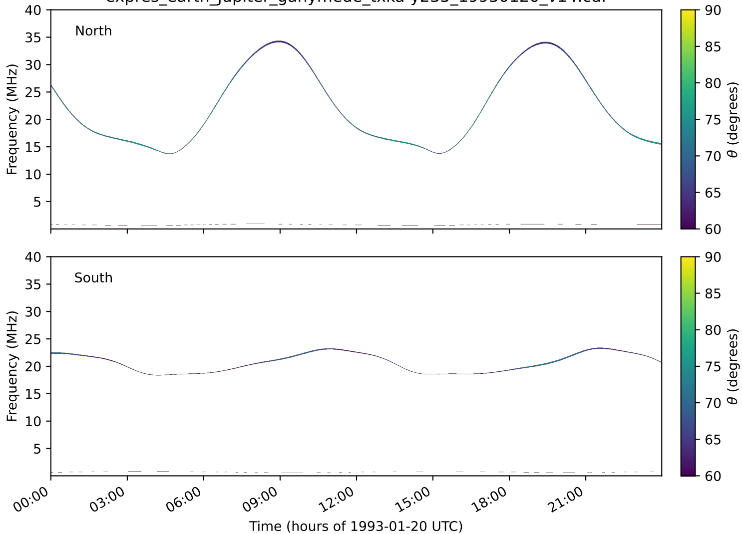
expres_earth_jupiter_ganymede_txka-y235_19930120_v14.cdf
