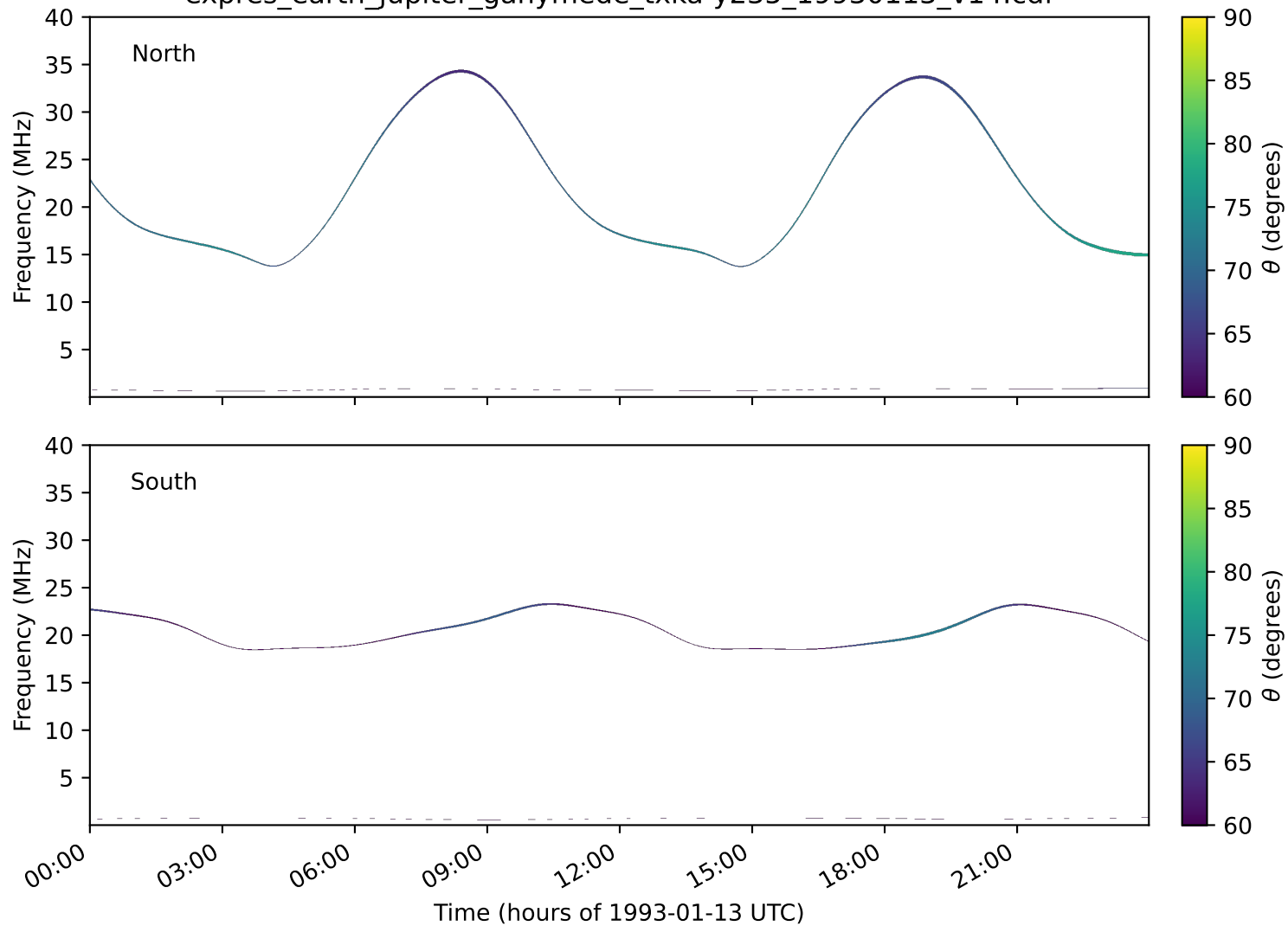
expres_earth_jupiter_ganymede_txka-y235_19930113_v14.cdf
