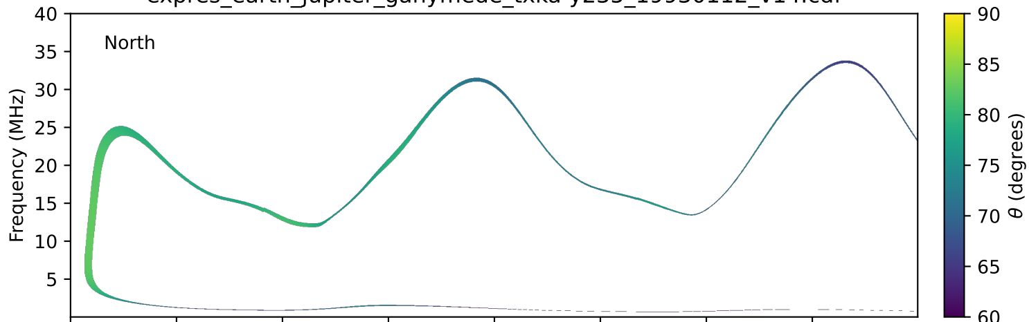
expres_earth_jupiter_ganymede_txka-y235_19930112_v14.cdf
