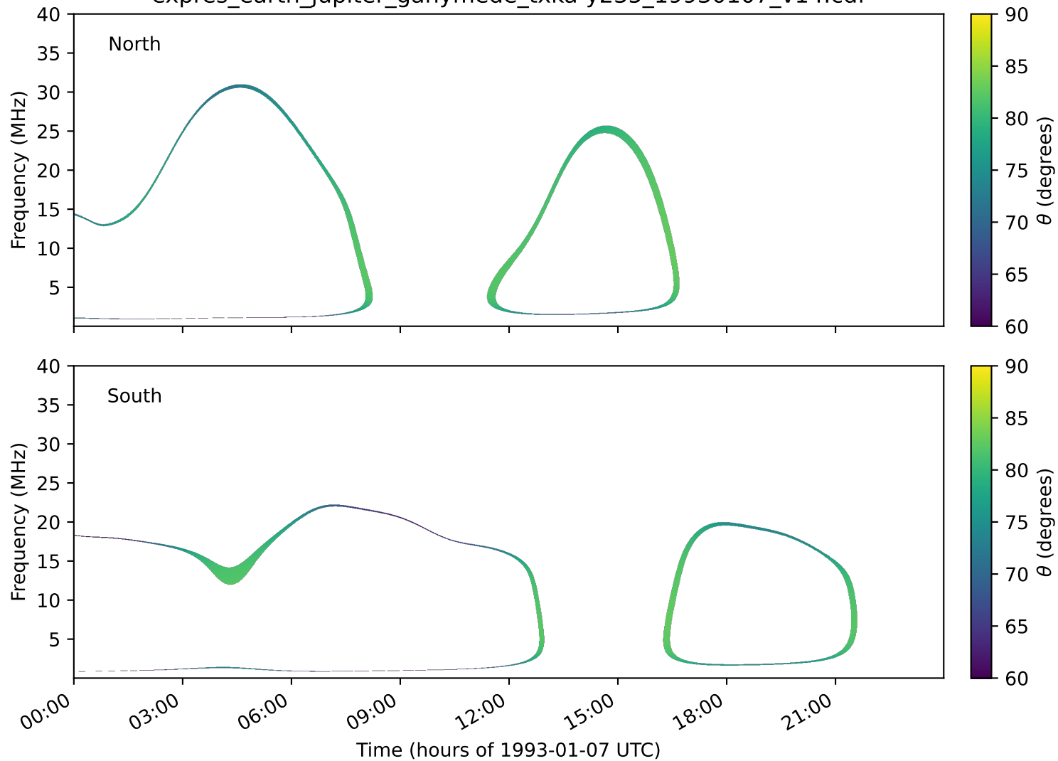
expres_earth_jupiter_ganymede_txka-y235_19930107_v14.cdf
