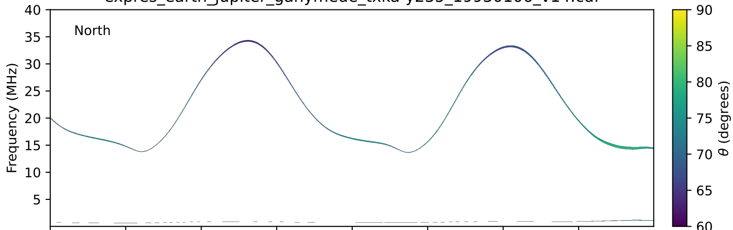
expres_earth_jupiter_ganymede_txka-y235_19930106_v14.cdf
