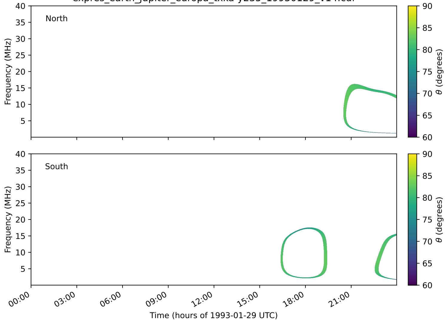
expres_earth_jupiter_europa_txka-y235_19930129_v14.cdf
