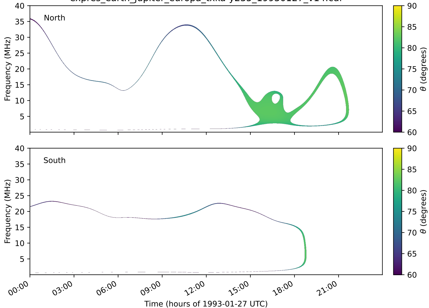
expres_earth_jupiter_europa_txka-y235_19930127_v14.cdf
