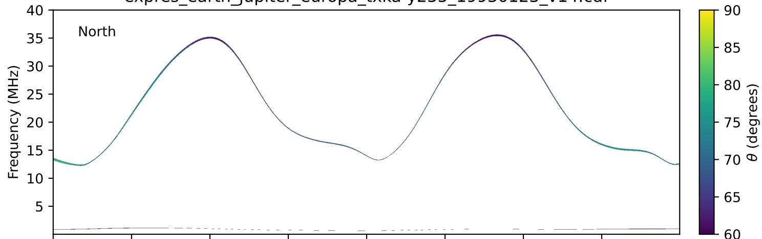
expres_earth_jupiter_europa_txka-y235_19930123_v14.cdf
