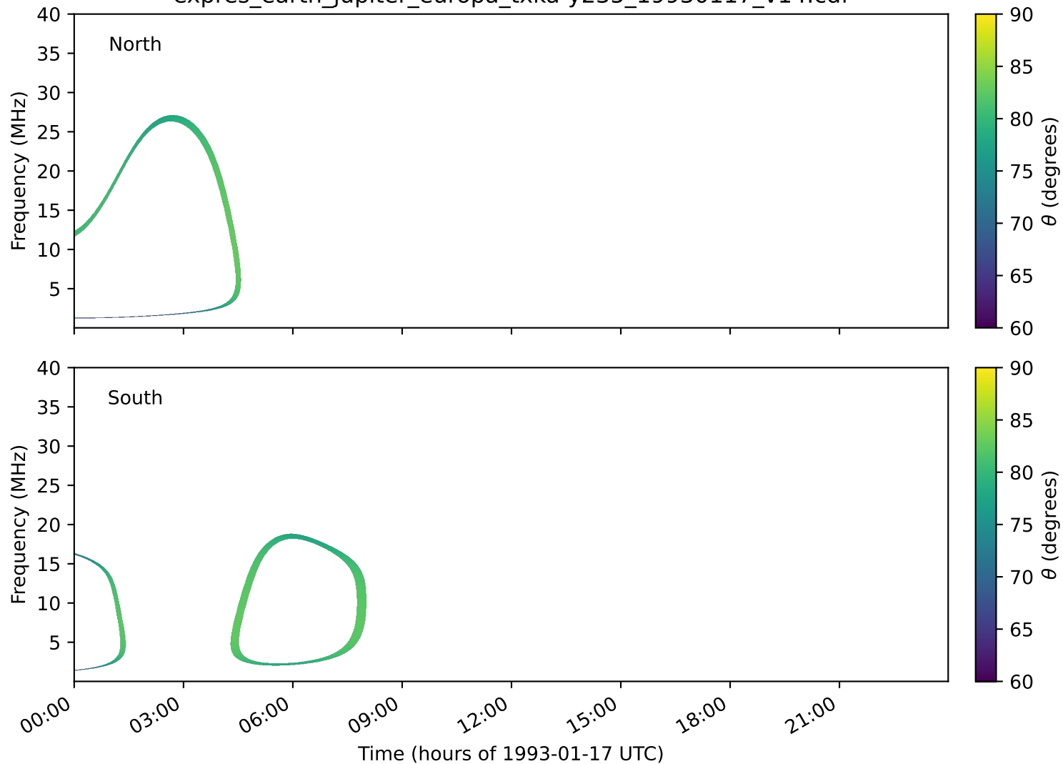
expres_earth_jupiter_europa_txka-y235_19930117_v14.cdf
