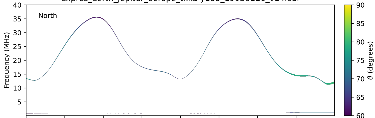
expres_earth_jupiter_europa_txka-y235_19930116_v14.cdf
