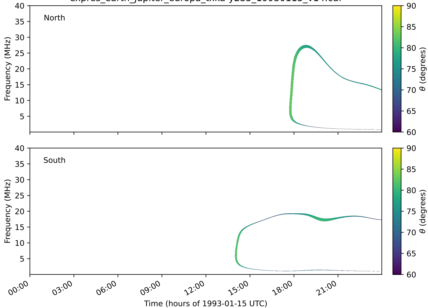
expres_earth_jupiter_europa_txka-y235_19930115_v14.cdf
