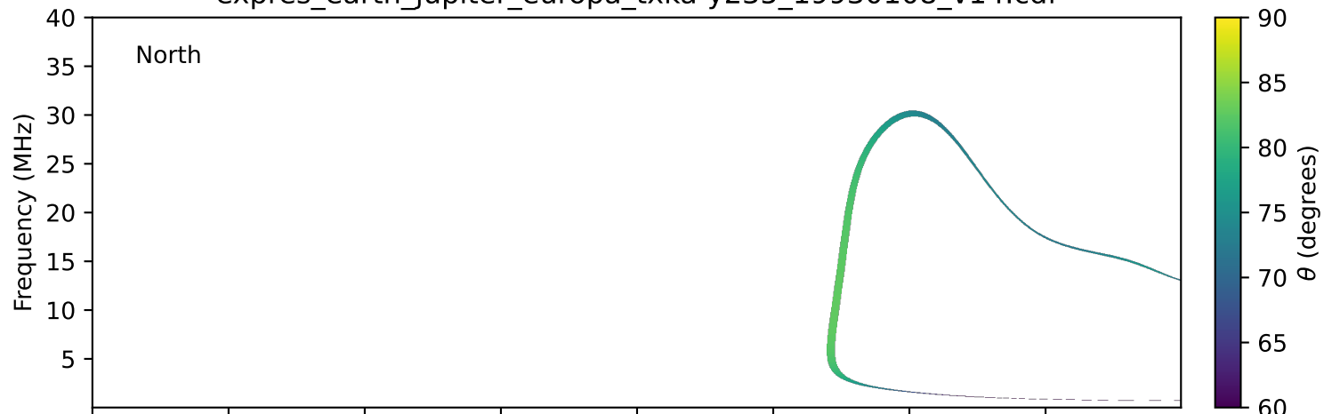
expres_earth_jupiter_europa_txka-y235_19930108_v14.cdf
