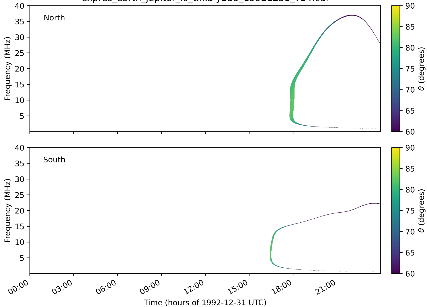
expres_earth_jupiter_io_txka-y235_19921231_v14.cdf
