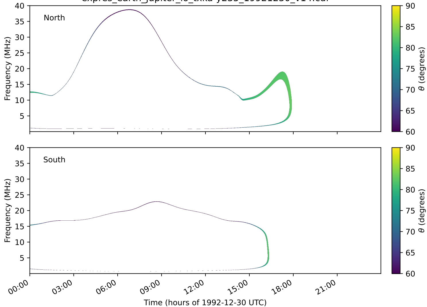
expres_earth_jupiter_io_txka-y235_19921230_v14.cdf
