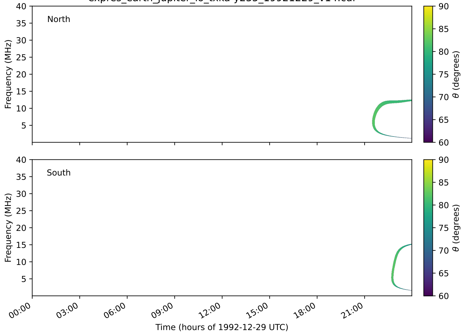
expres_earth_jupiter_io_txka-y235_19921229_v14.cdf
