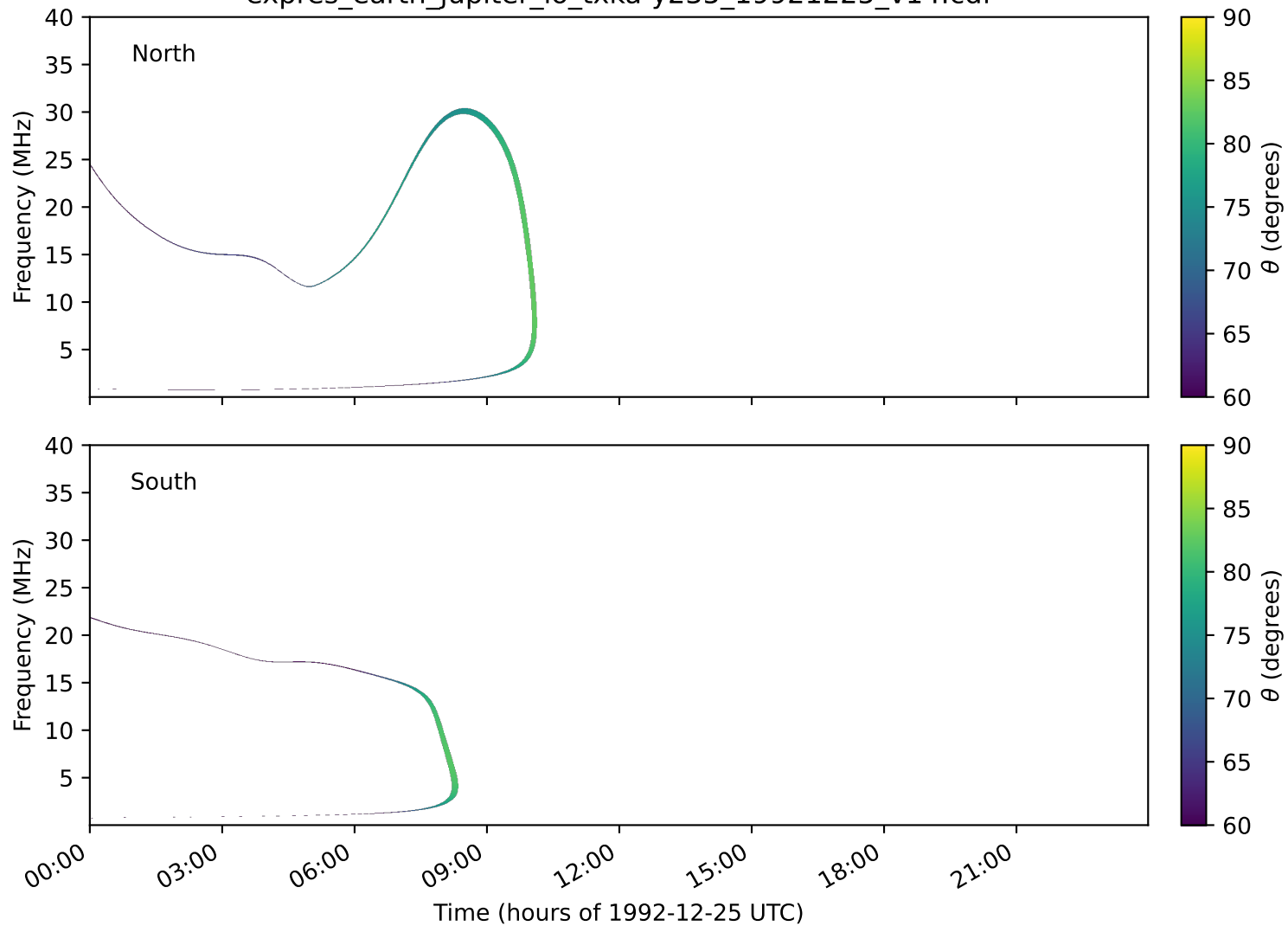
expres_earth_jupiter_io_txka-y235_19921225_v14.cdf
