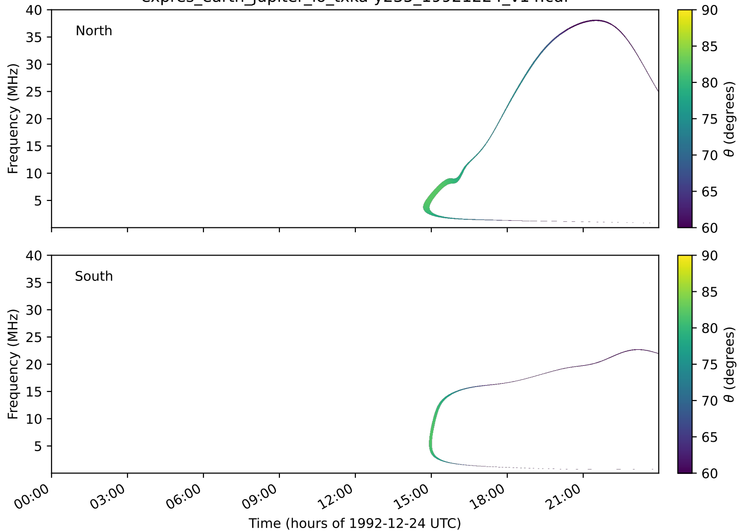
expres_earth_jupiter_io_txka-y235_19921224_v14.cdf
