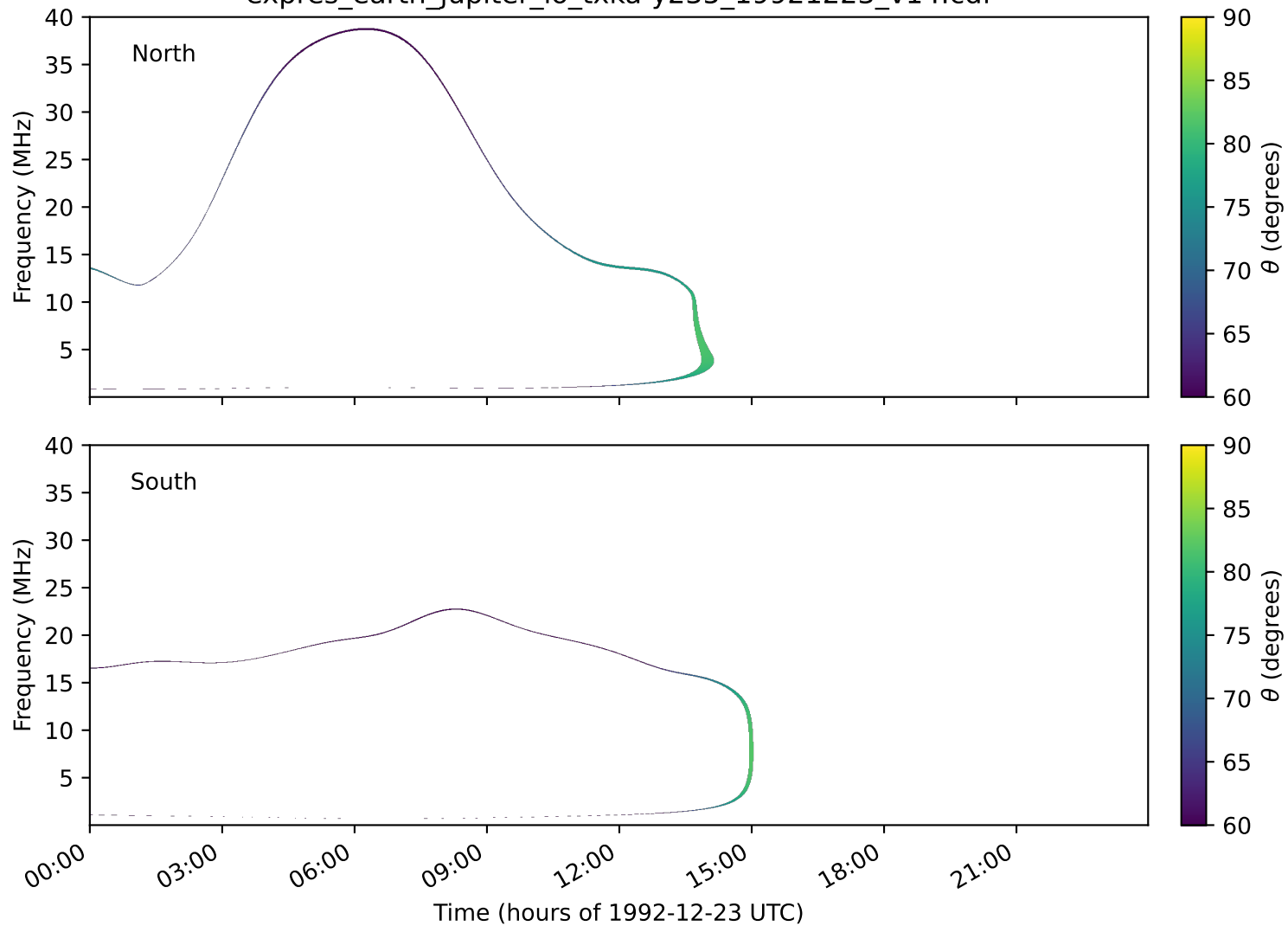
expres_earth_jupiter_io_txka-y235_19921223_v14.cdf
