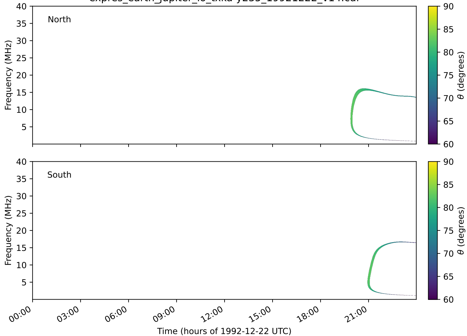
expres_earth_jupiter_io_txka-y235_19921222_v14.cdf
