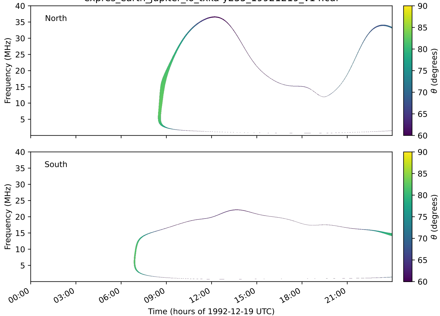
expres_earth_jupiter_io_txka-y235_19921219_v14.cdf
