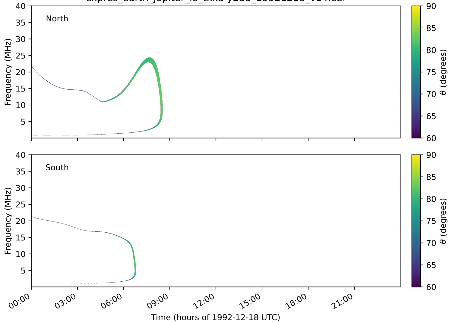
expres_earth_jupiter_io_txka-y235_19921218_v14.cdf
