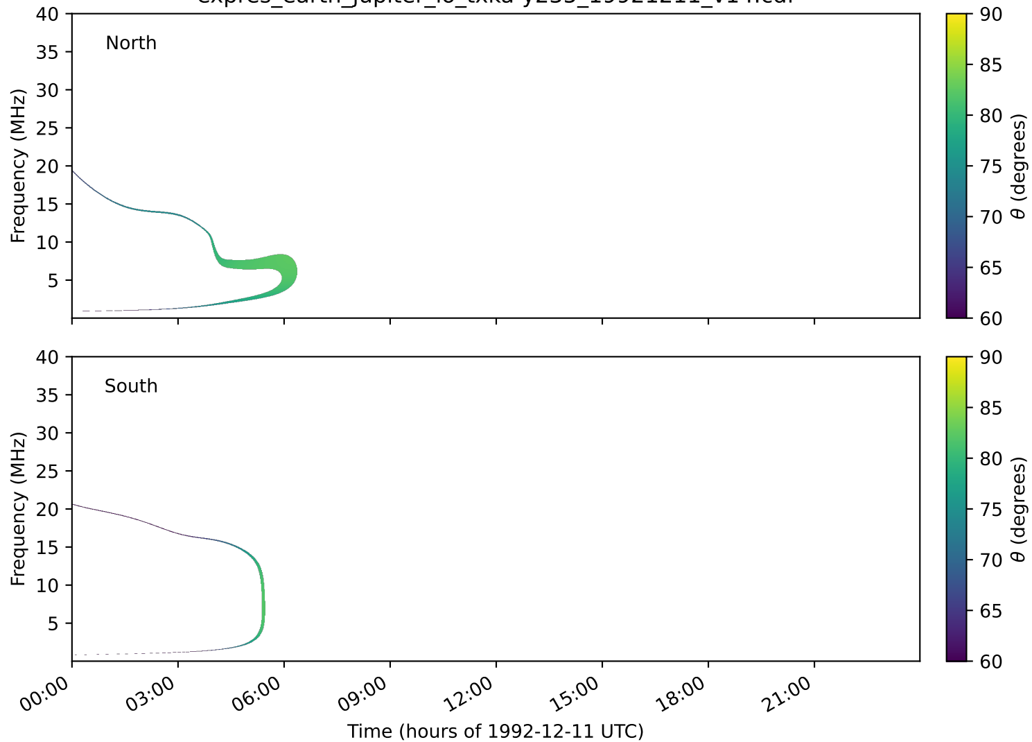
expres_earth_jupiter_io_txka-y235_19921211_v14.cdf
