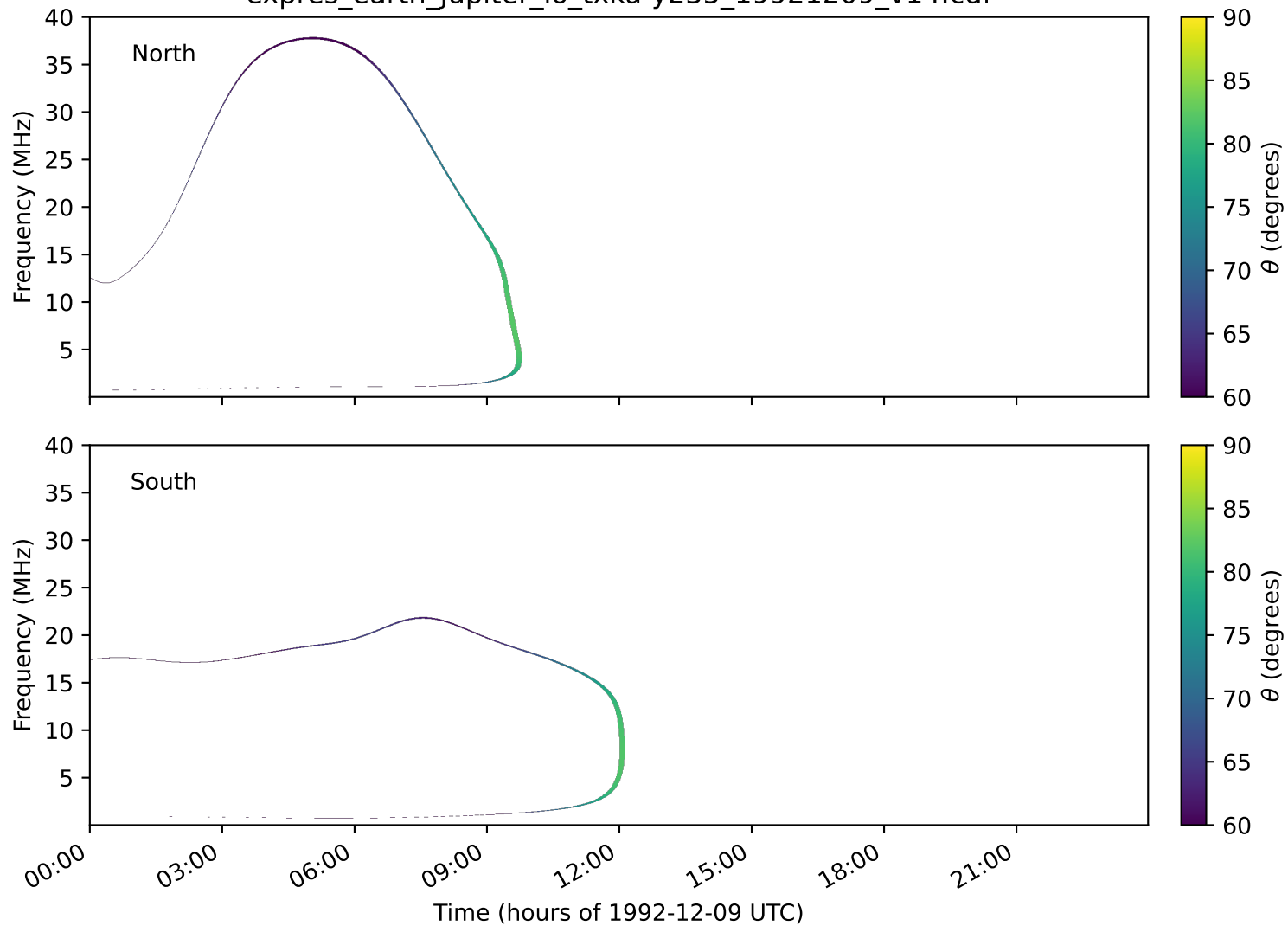
expres_earth_jupiter_io_txka-y235_19921209_v14.cdf
