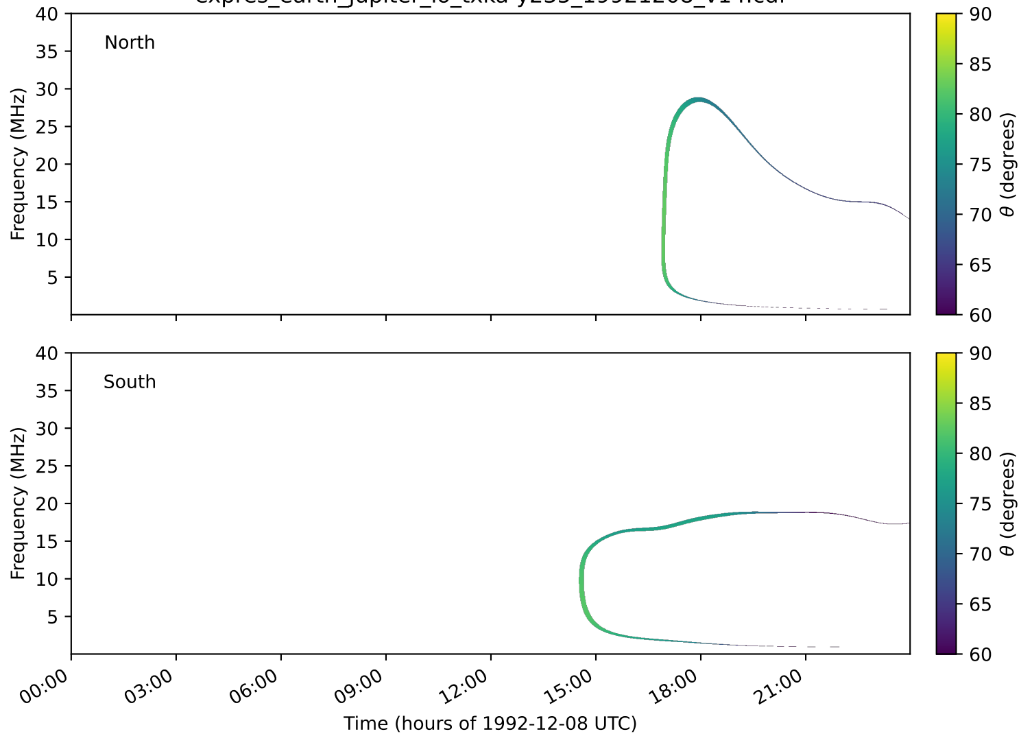
expres_earth_jupiter_io_txka-y235_19921208_v14.cdf
