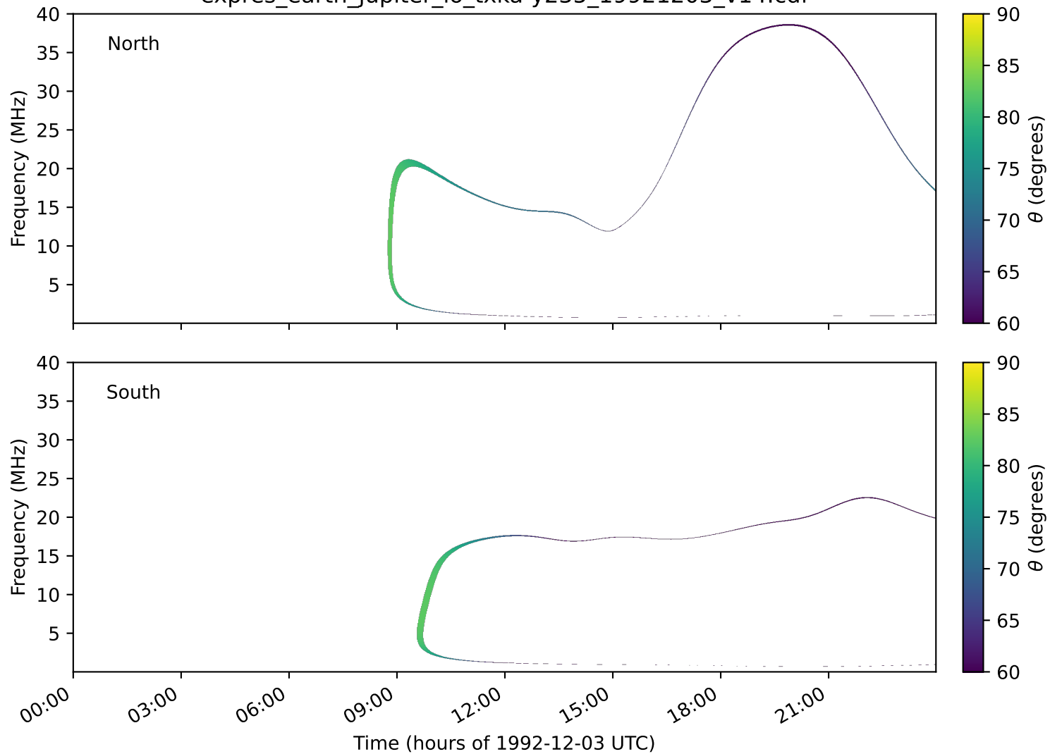
expres_earth_jupiter_io_txka-y235_19921203_v14.cdf
