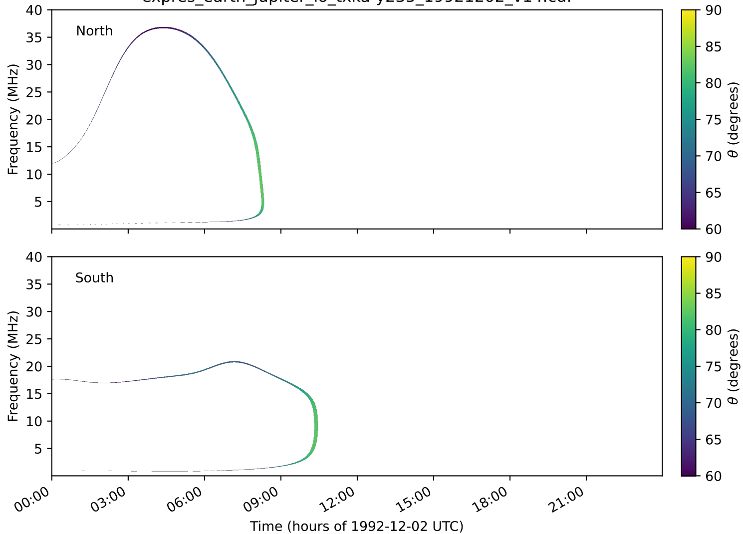
expres_earth_jupiter_io_txka-y235_19921202_v14.cdf
