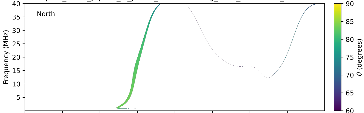
expres_earth_jupiter_io_jrm33_lossc-wid1deg_3kev_19921219_v11.cdf
