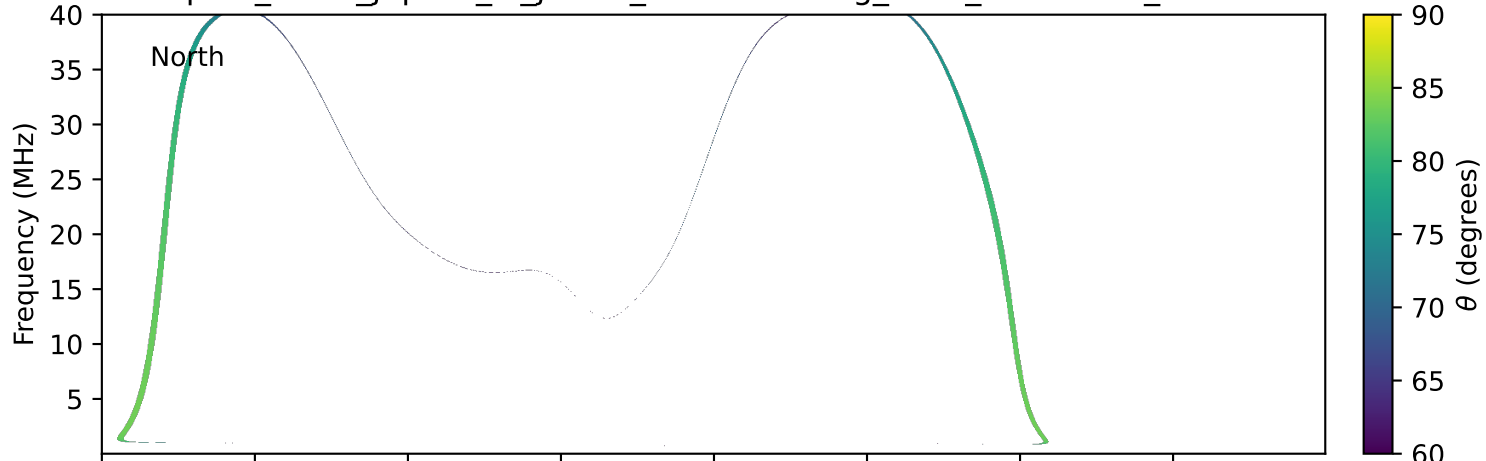
expres_earth_jupiter_io_jrm33_lossc-wid1deg_3kev_19921214_v11.cdf
