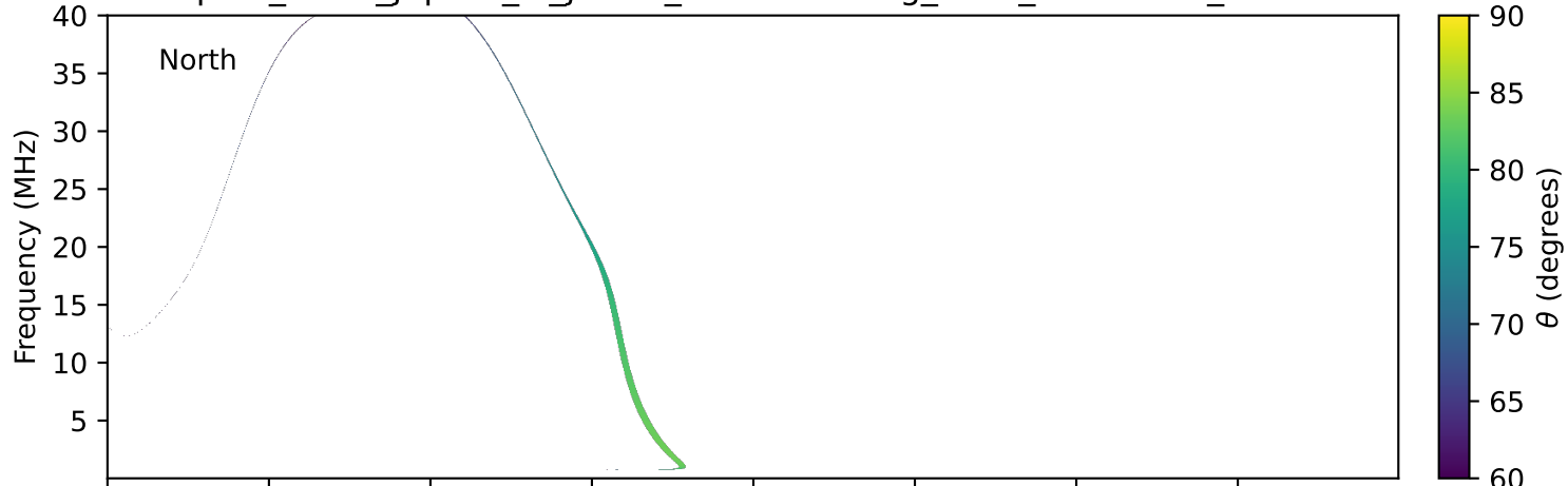
expres_earth_jupiter_io_jrm33_lossc-wid1deg_3kev_19921209_v11.cdf
