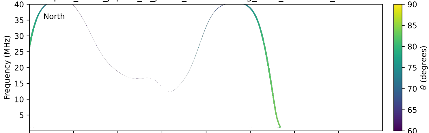
expres_earth_jupiter_io_jrm33_lossc-wid1deg_3kev_19921207_v11.cdf
