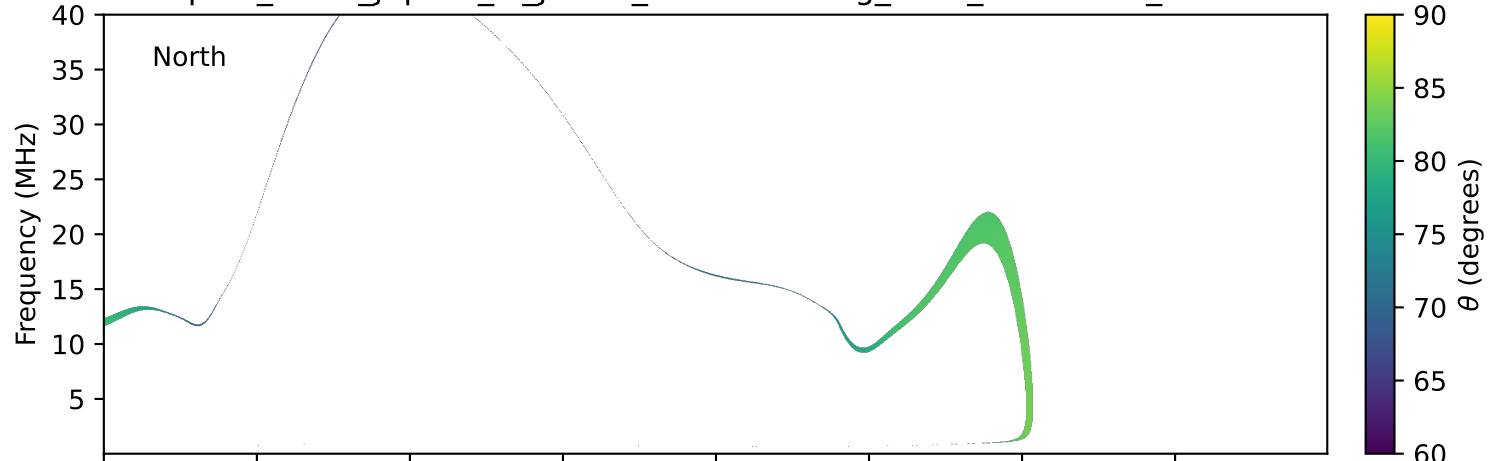
expres_earth_jupiter_io_jrm09_lossc-wid1deg_3kev_19921230_v11.cdf
