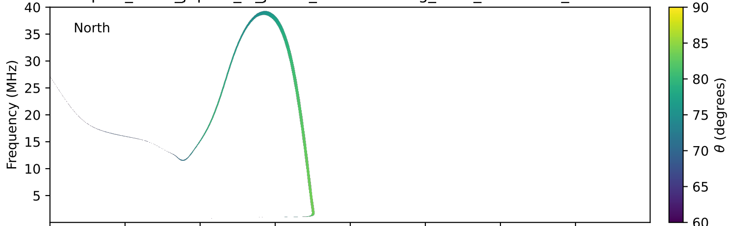
expres_earth_jupiter_io_jrm09_lossc-wid1deg_3kev_19921225_v11.cdf
