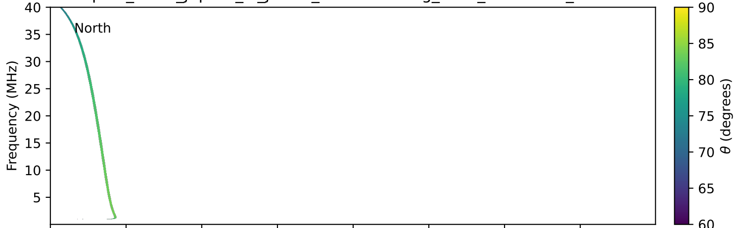
expres_earth_jupiter_io_jrm09_lossc-wid1deg_3kev_19921220_v11.cdf
