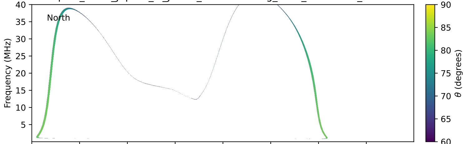
expres_earth_jupiter_io_jrm09_lossc-wid1deg_3kev_19921214_v11.cdf
